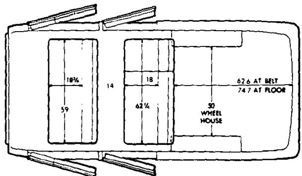
Front, Folding Center And Rear Removable Seats Standard front, RPO AT5 folding center and RPO A53 removable rear seats
